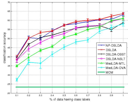
Fig. 3. p_1 = 0.5 (Conference)
