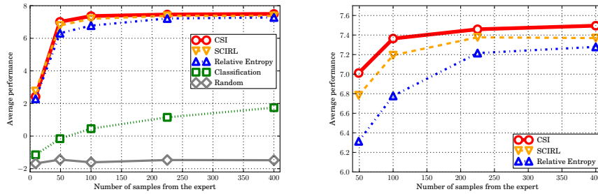
(a) Mean performance over 100 runs on the (b) Zoom of Fig 2a showing the ranking of Highway driving problem. the three IRL algorithms.
