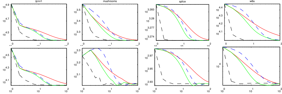
Fig. 2. (Medium-size real data) The top and bottom rows correspond to training and test data, resp. The x-axis measures iterations, and the y-axis measures loss with and without regularization for the training and test sets, resp.
