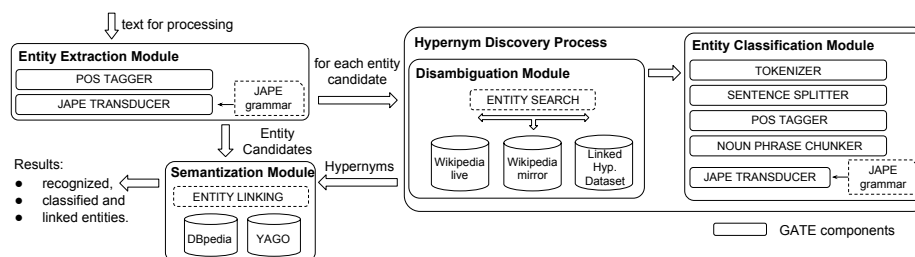
Fig. 1. Architecture overview
